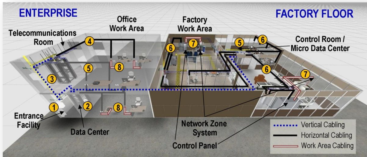
Figure 1. Structured Cabling Block Diagram.
