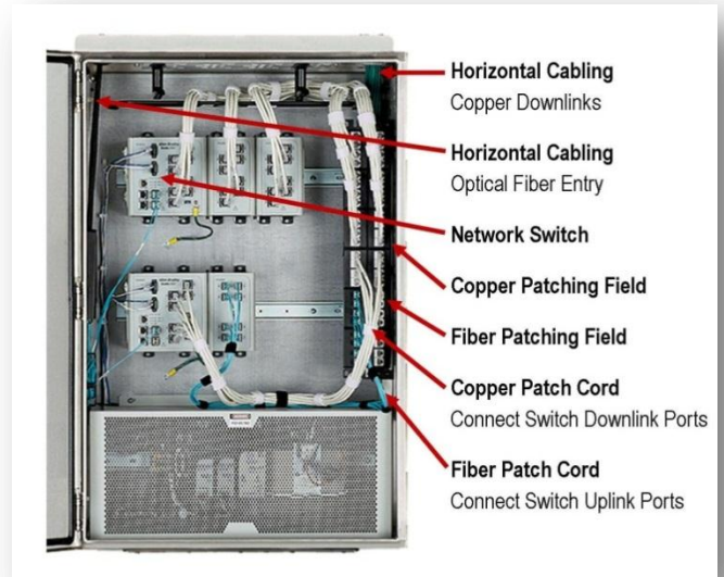
Figure 4. Integrated Network Zone System permanent link implementation.
