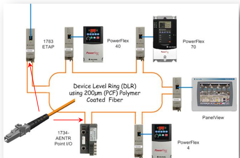
Figure 5. Device Level Schematic of a Fiber Point to Point Cabling System.
